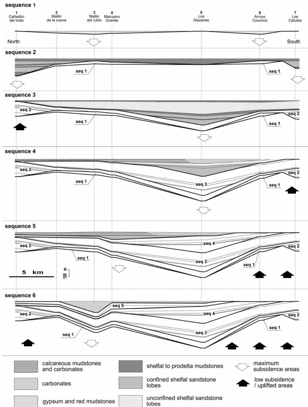
FIGURE 9 | Diagram showing the progressive accumulation of the Lotena Group in the Sierra de la Vaca Muerta, with indication of the main facies types. White arrows for each sequence show the location of areas of low topographic relief, attributed to greater subsidence rates at time of deposition, while black arrows indicate the location of areas experienced less subsidence or uplift. Note the progressive northward shift of sequences 4 to 6 depocentres. Numbers on top refer to stratigraphic sections (see Fig. 2 for location).
