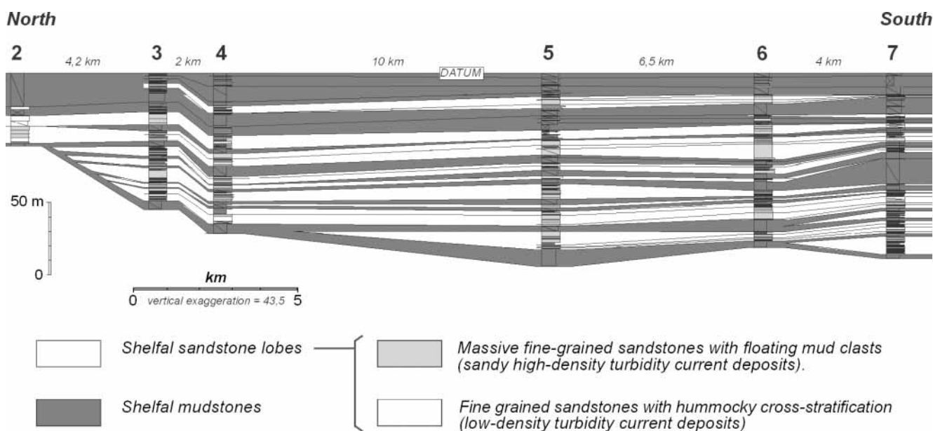
FIGURE 6 | Detailed cross section of unconfined shelfal sandstone lobes of sequence 3, along a distance of about 26,7 km in a direction roughly perpendicular to paleocurrent directions. These strata are composed of fine-grained and normal-graded sandstone bodies, which appear massive or having hummocky cross-stratification. Paleocurrents are from the southwest. See Fig. 2 for location of the sections.
